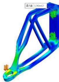
3DCAD
